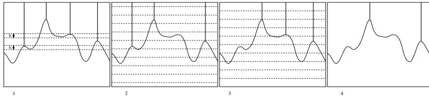
Fig. 4. The second cause of over-segmentation in the watershed: poor dynamics minima. Basins of depth inferior to h (1) are discarded thanks to the Buffon's method (2), (3), (4).
