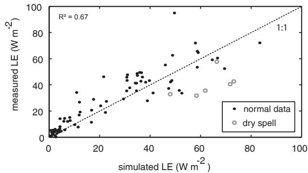
Figure 5. A one-to-one comparison of weekly averages of latent heat (LE) for the POPFULL site, between the model outputs and the measured values. The dotted line is the 1 : 1 line. Weeks 18–23, which represent the dry spell, are highlighted as grey circles.
