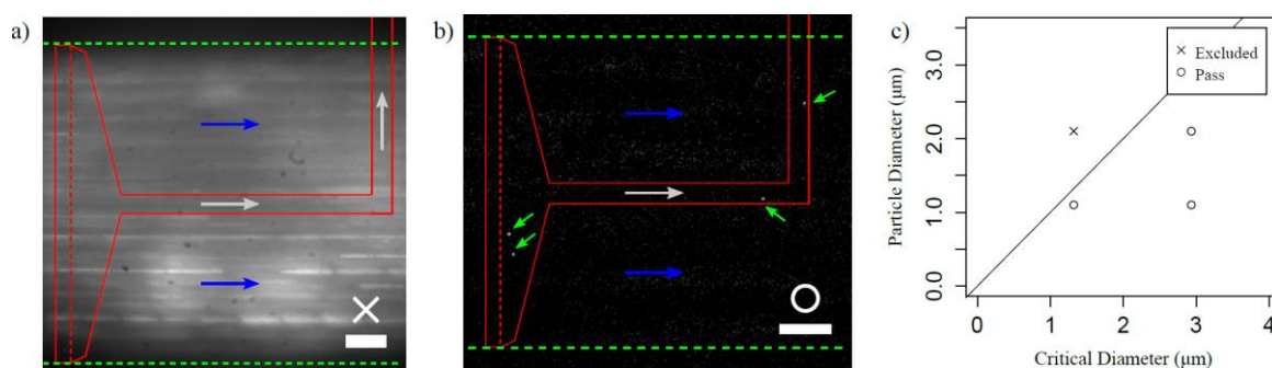
Figure 7- Experimental results obtained with the 3D device. (a-b) Micrographs of exclusion or aspiration of 1 or 2 \mu\text{m} diameter beads for a 1.3\ \mu\text{m} critical diameter. Scale bars are 50\ \mu\text{m} . Pressure difference between inlet and outlets is 10 mbars. The particles are flowing from left to right: arrows symbolize the flow in the main outlet channel (blue arrows) and in the lateral channel (light grey arrows). (a) 2\ \mu\text{m} (red fluorescent) particles are flowing in the main channel and do not enter in the lateral channel. (b) 1\ \mu\text{m} (green fluorescent) particles flow in both main and lateral channels (green arrows point at particles). (c) Summary of experimental results for two sizes of beads, obtained with one device operated with different output/lateral pressures enabling to tune the partial flow rate Q^* (see Equation 4), and thus the critical diameter. Horizontal axis shows the critical diameter d_c of the device for specific applied pressures: d_c = 1.3\ \mu\text{m} for \Delta P^* = 1 and d_c = 2.9\ \mu\text{m} for \Delta P^* = 1/3 . If during an experiment, particles flow through the side channel, the experiment is represented as an o. If no particle is entering the side channel, the experiment is represented as an x.
