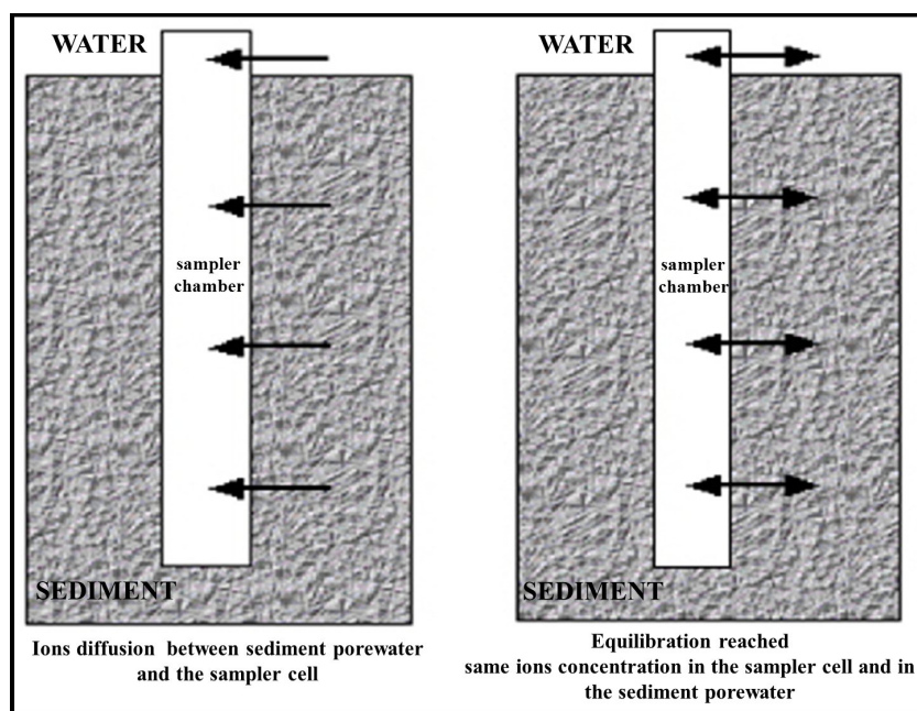
Figure 1. Principle of the porewater sampler
