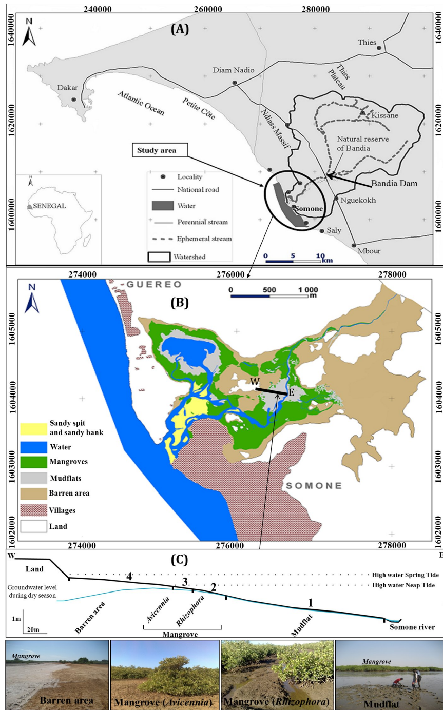
Figure 5. Study site. A : location of the Petite Côte of Senegal; B : estuary and lagoon; C : cross-section of the geomorphological units of the Somone estuary; bottom : profile photographs corresponding to the points indicated on the above cross-section.
