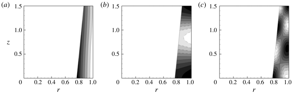
FIGURE 16. Structure of some waves in the top-wall case for m = 2, a = 0.5, a_t = 1.5, Ek = 10^{-4}, Fr = 6 . (a) C_0^- ; \lambda_r = -0.576, \lambda_i = -0.00101 ; (b) C_2^+ ; \lambda_r = 2.256, \lambda_i = -0.00716 ; (c) I_{31}^- ; \lambda_r = -0.644, \lambda_i = -0.0387 .
