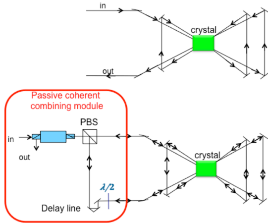
Fig. 2. Implementation of the passive coherent combining in a geometrical multipass amplifier based on a Sagnac interferometer. The use of a PBS (polarizer beam splitter) and a half-wave plate allows the use of a polarization-sensitive amplifier. The delay line has the role of avoiding temporal overlap of the two counter-propagating beams in the crystal.
