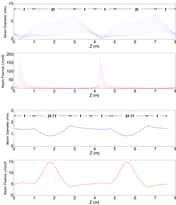
Fig. 10. Beam propagation simulation. Beam diameter evolution (blue curve) and intracavity fluence for 100 mJ pulses (red curve) without (upper part) and with (lower part) thermal lens compensation. In the second case all the curves are almost perfectly overlapped.
