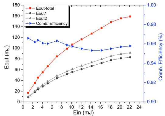
Fig. 13. Performance of the coherent combining of a high energy multipass amplifier. A total energy of 160 mJ is obtained at maximum with 96% of efficiency in the beam combining process.
