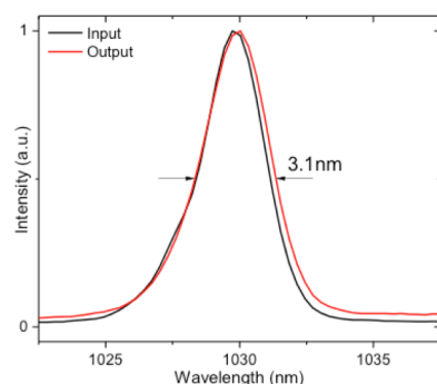
Fig. 15. Spectra before and after amplification demonstrating the absence of gain narrowing (corresponding FLT of <500 fs).
