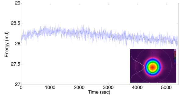
Fig. 11. Beam profile and stability of the double head multipass amplifier operating at 100 Hz. The input energy of the amplifier is adjusted for security reasons to fix the output at 28 mJ and the measurement is performed over 1 \frac{1}{2} hours.
