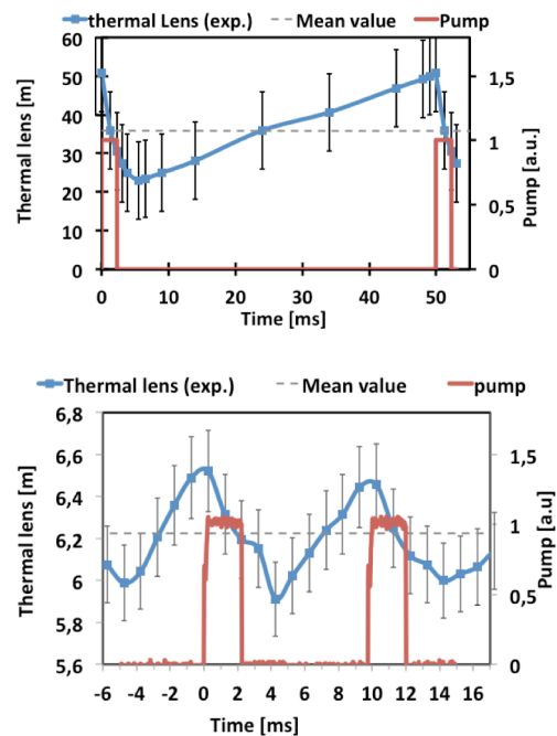
Fig. 9. Experimental measurements of the thermal lens at 20 Hz (top- and 100 Hz (bottom).
