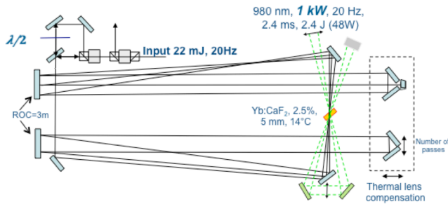
Fig. 12. Experimental setup of the amplifier using coherent combining.
