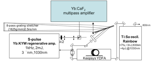
Fig. 3. Experimental setup for the generation of the input beam for the multipass amplifiers.
