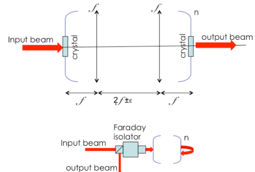
Fig. 1. Reimaging multipass amplifier principle with thermal lens compensation (top) and recycling principle (bottom).
