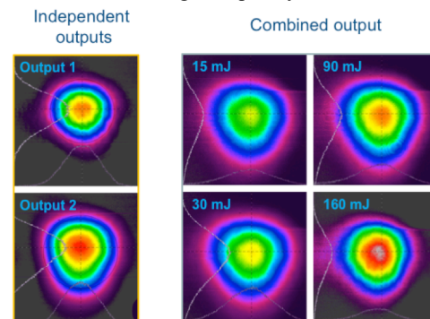
Fig. 14. Beam profiles of the two counter-propagating beams measured independently (left). Beam profiles of the beam after combining for different output energy (right).
