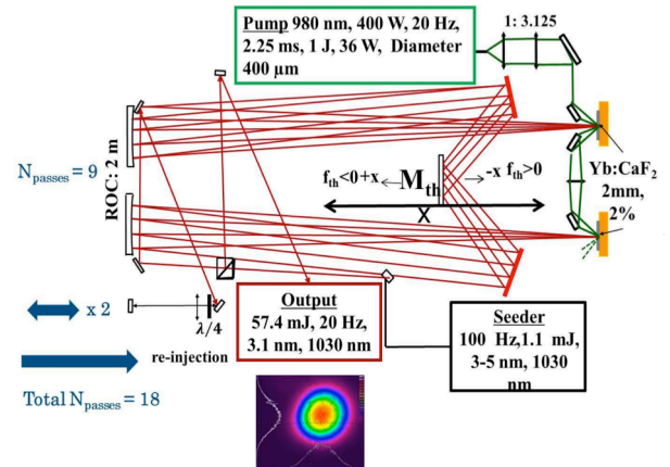
Fig. 8. Experimental setup of the re-imaging multipass amplifier with two Yb:CaF 2 active-mirrors.
