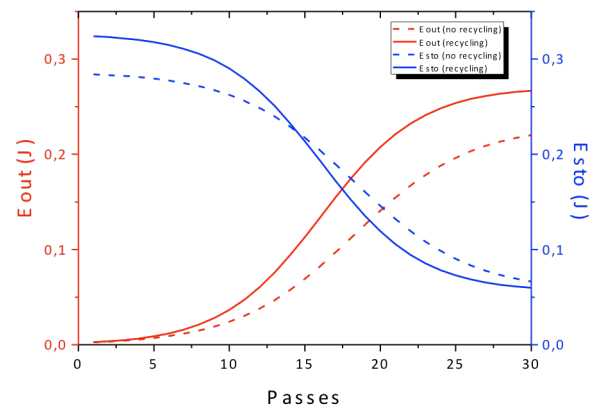
Fig. 4. Numerical simulations for a 2.5 % 5-mm-long Brewster-angle-cut crystal pumped with 1.2 J on a 1.5 mm diameter without (dashed lines) or with (solid lines) pump recycling.
