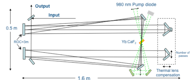
Fig. 6. Experimental setup using a 2.5% 5-mm-long Brewster-oriented crystal pumped with 1.2 J on a 1.5 mm diameter.
