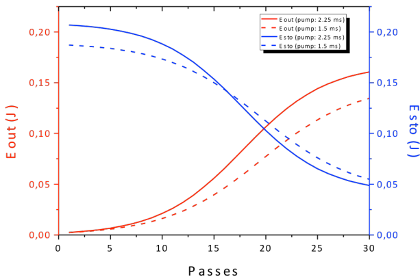
Fig. 5. Numerical simulations for two 2.2%-doped, 2-mm-long active-mirror crystals pumped with 0,9-J 2.25-ms pumping (solid lines) and 0,6-J, 1,5-ms pumping (dashed lines) both for a 1.5 mm diameter 2-mJ input signal beam.
