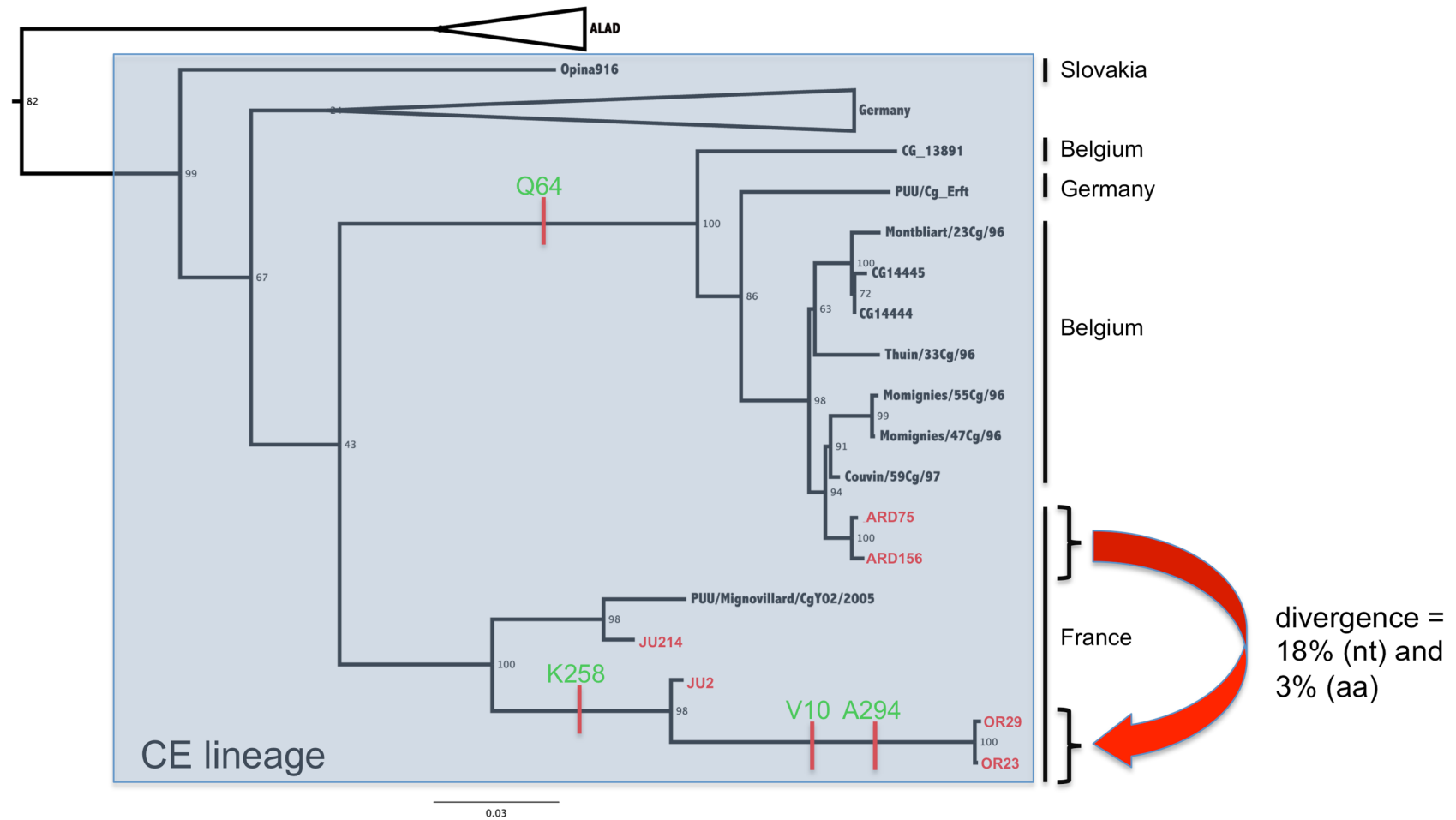
Figure 2. Phylogenetic tree based on the complete N protein coding sequences (the S segment N- ORF) of PUUV of the central European (CE) lineage. Scale bar represent the average number of substitutions per site. French isolates from this study are in red and specific amino acid (aa) signatures are indicated on the branches of the tree.
