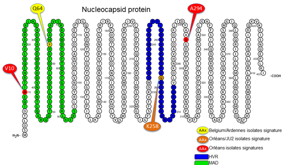
Figure 4. PUUV nucleocapsid protein aa sequence visualized with Protter—visualize proteoforms [31]. The used aa sequence corresponds to the consensus sequence of the S sequences dataset. The major antigenic domain (MAD) is represented in green and the hyper variable region (HVR) in blue.
