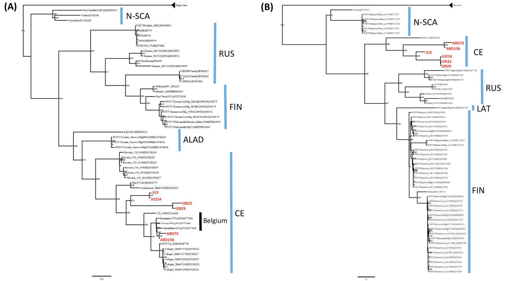
Figure 3. Phylogenetic trees based (A) on the partial (2484–3010 nt) M segment sequences and (B) on the partial (577–989 nt) L segment sequences of PUUV. Scale bar represent the average number of substitutions per site. French isolates are in red. Blue bars indicate known PUUV lineages.
