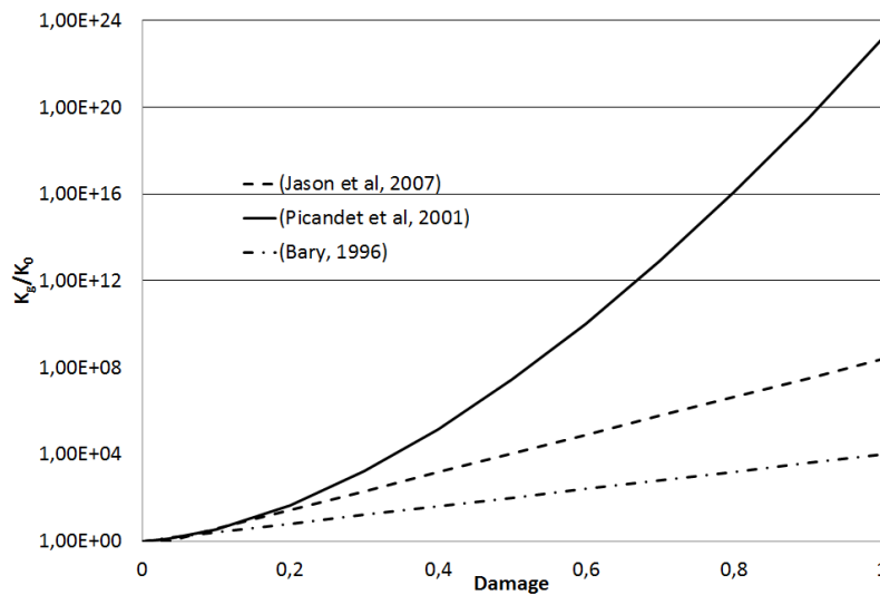
Figure 10. Damage-permeability laws
