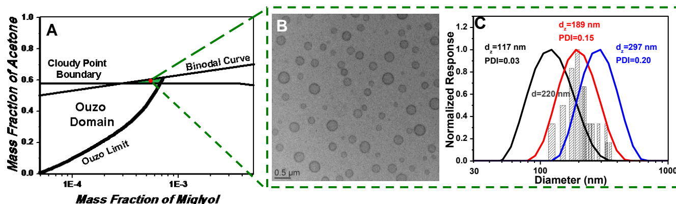
Figure 1: (A) Overlapped phase diagrams of P(HMM 206 -stat-GMA 17 ) and miglyol in acetone/water mixtures. The domain in which nanocapsules can be generated through co-nanoprecipitation of miglyol and glycopolymer corresponds to the green zone of Fig 1A. Accordingly, nanoprecipitations were performed in the following conditions: polymer content = 0.025 wt %, miglyol content = 0.05 wt %, acetone content = 59 wt %. (B) TEM picture of the resulting glyconanocapsules (C) Comparison of DLS (from left to right, analyses performed in the conditions given in (A), Dulbecco's PBS buffer and distilled water) and TEM size distribution (histogram).
