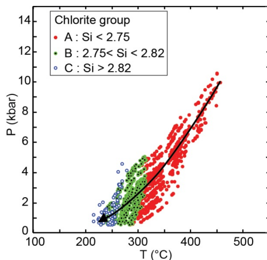
Fig. 10. P – T diagram presenting the chemical composition of chlorite vs. P – T equilibrium conditions. The black arrow shows a P – T path consistent with multi-equilibria calculations. Each point on the P – T diagram represents equilibrium conditions for one chlorite composition, equilibrated with one white mica composition (Table 4) using the multi-equilibria method described in Appendix S2.
