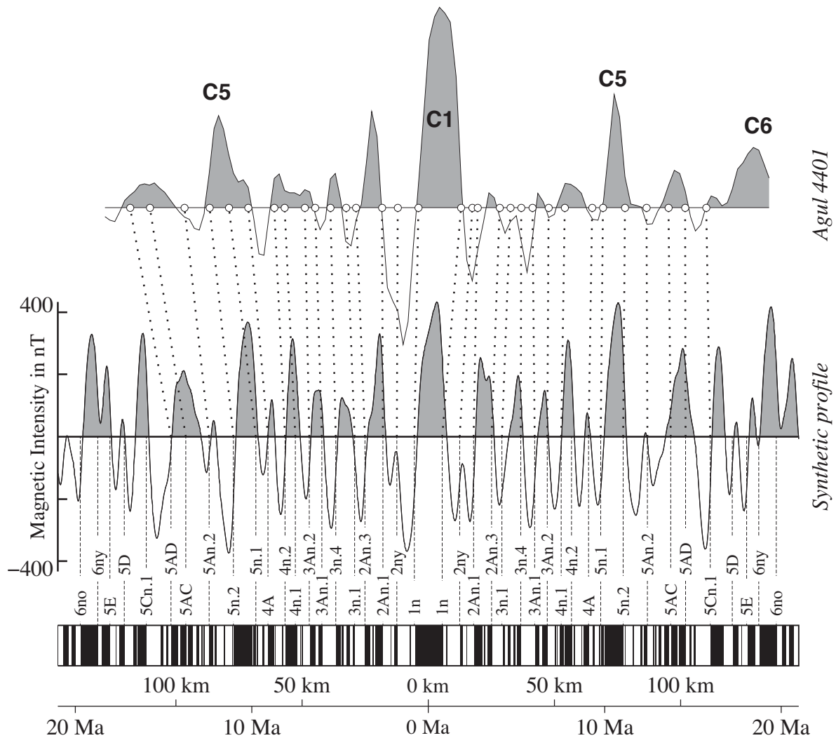
Figure 3. Comparison of magnetic anomaly profile from the Agulhaus 4401 survey of the Southwest Indian Ridge, 21^{\circ}\text{E} to 24^{\circ}\text{E} , to a synthetic magnetic profile created using a 14\text{ mm yr}^{-1} spreading rate, a ridge azimuth of \text{N}75^{\circ}\text{W} , a 500-m wide reversal transition zone, and ambient and paleomagnetic inclinations and declinations appropriate for the survey area. The magnetic block model and magnetic reversal correlation points (dotted lines) used for this study are shown below the synthetic magnetic anomaly profile.
