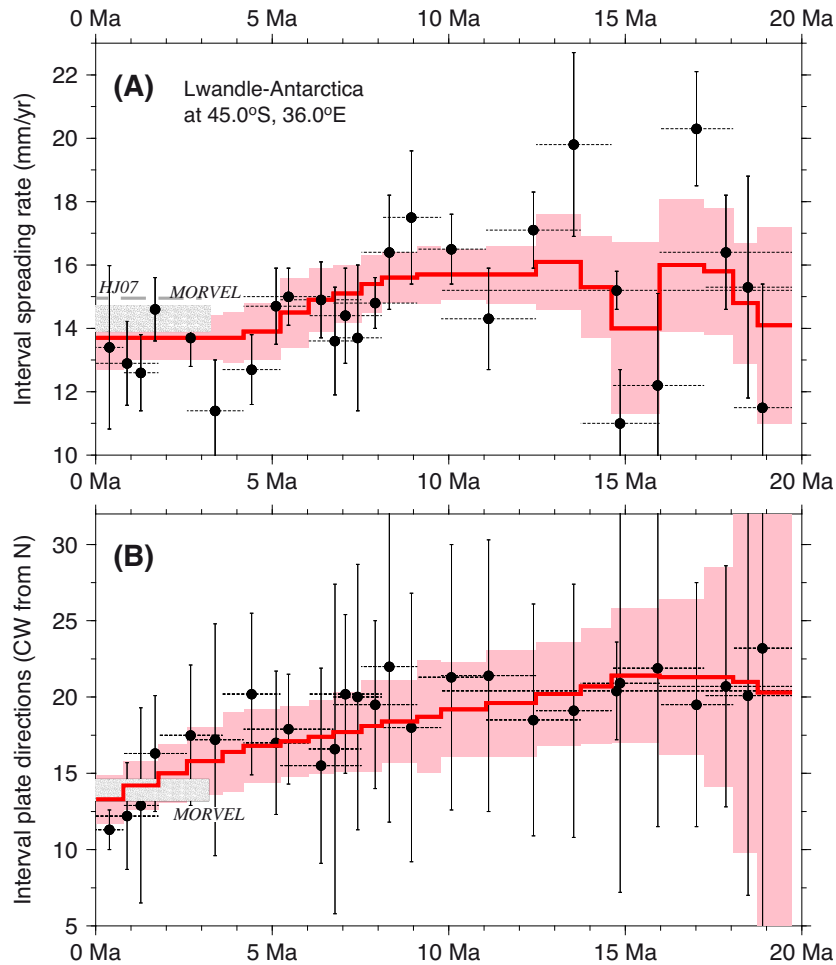
Figure 22. Lwandle–Antarctic plate interval velocities at 45.0°S, 36.0°E. Black circles show interval rates and directions determined from stage rotations that we derived from the best-fitting finite rotations in Table 3. These average plate motion over 1-Myr-long to 3-Myr-long intervals, as indicated by the horizontal dashed lines that are centred on the circles. The red line and pink-shaded area show interval velocities and nominal 1- \sigma uncertainties determined with the noise-reduced stage rotations from Supporting Information Table S5. (A) Interval seafloor spreading rates. Grey bar is centred on the 3-Myr-average MORVEL Lwandle–Antarctica estimate and encompasses its 1- \sigma uncertainty. The interval rates use magnetic reversal age estimates from Table 1. ‘HJ07’ identifies the 3-Ma-average rate predicted by the Lwandle–Antarctic angular velocity of Horner-Johnson et al. (2007). (B) Lwandle–Antarctica interval directions. Grey bar shows the MORVEL estimate and encompasses its 1- \sigma directional uncertainty.
