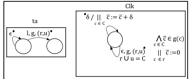
Fig. 1. Semantics of TA via a Composition of Two LTSs
