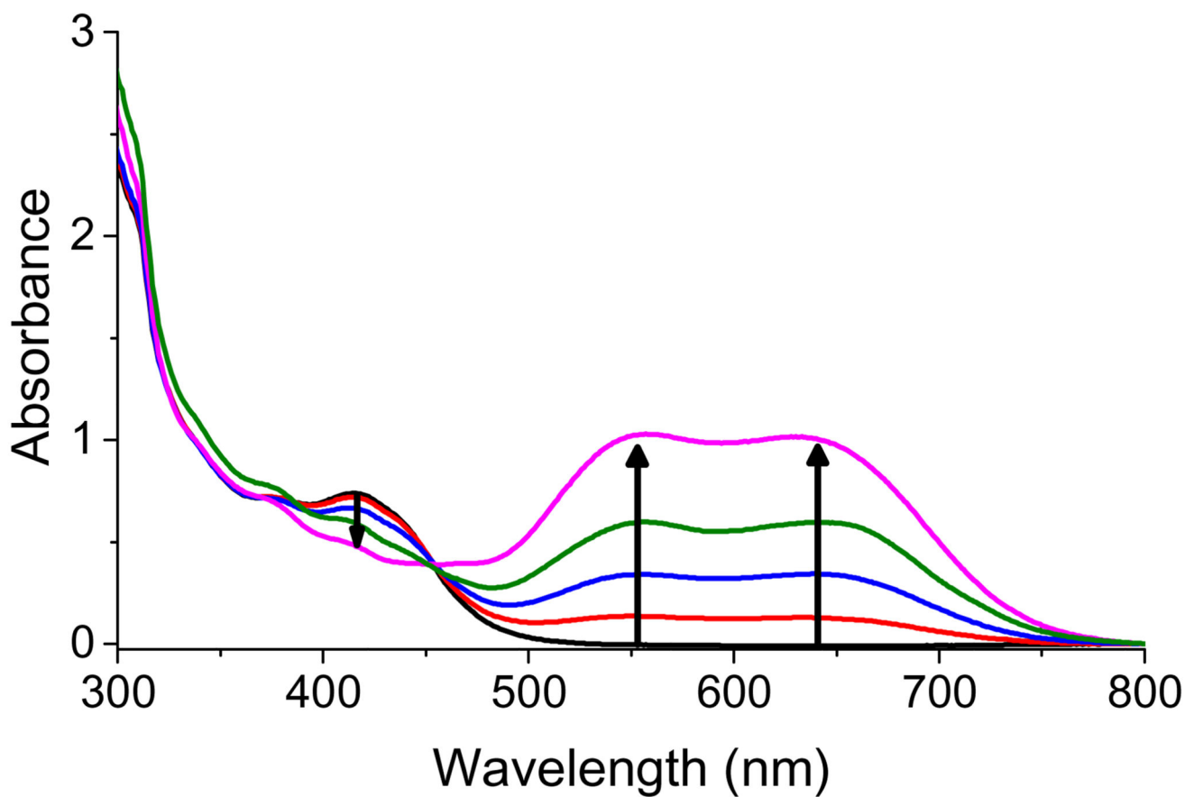
Figure 3. UV-Vis spectra recorded before (black line) and after 30 s (red line), 1 minute (blue line), 2.5 minutes (green line) and 5 minutes (magenta line) of visible light irradiation on anhydrous \text{CH}_3\text{CN} solutions of \text{Co}2 and [\text{Ir}(\text{ppy})_2(\text{bpy})](\text{PF}_6) in the presence of TEOA (5 %). The transition \text{Co}(\text{II}) \rightarrow \text{Co}(\text{I}) is outlined by the appearance of a two-component signal.
