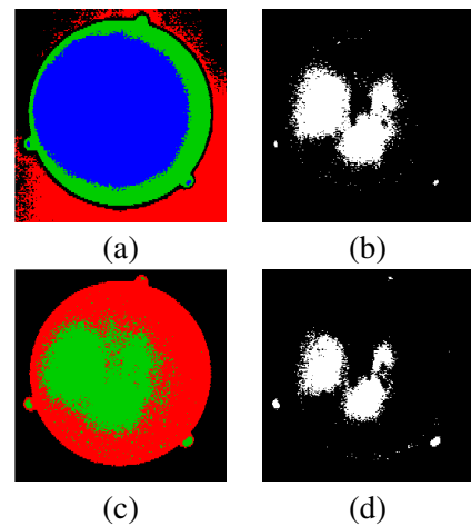
Fig. 8. (a) Clara segmentation in 4 clusters on parameter b , blue cluster is selected, (b) Clara on parameters a and m : parameters markers, (c) Clara segmentation in 4 clusters on parameter a , green cluster is selected, (d) Clara on parameters b and m : parameters markers.
