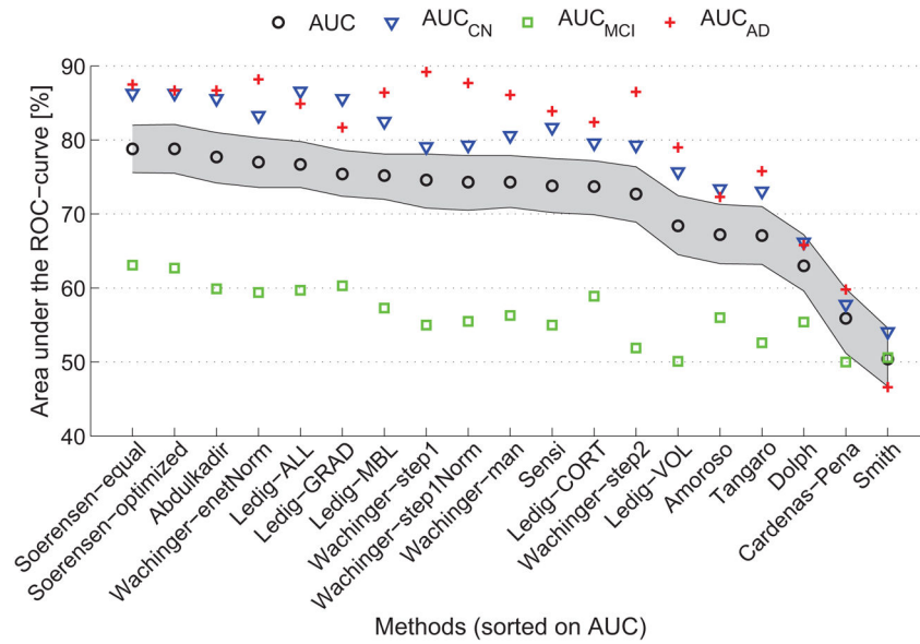
Figure 2. Area under the ROC-curve (AUC) on the test data for the participating algorithms. For total AUC, the 95% confidence interval is shown in grey.
