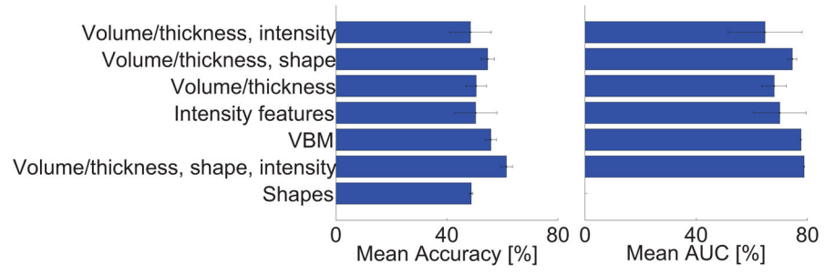
Figure 5. Mean accuracy and area under the ROC-curve (AUC) on the test data for the different types of features used by the algorithms. The error bars show the standard deviation.
