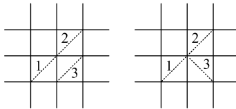
Figure 7: Local connections of the path when segments 1 and 2 are aligned. Left: segment 3 cannot be connected to the previous path of segments 1 and 2 due to its orientation; right: segment 3 with the converse orientation has a pending end point and the path cannot be closed. Conclusion: successive segments 1 and 2 cannot be aligned.
