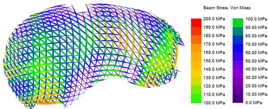
Figure 6: Stress resulting from forming in the Soliday's gridshell
