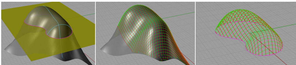
Figure 3: meshing process of a 3D surface. a. extension of the surface and drawing of the two curves. b. meshing of the extended surface. c. cutting of the useful part of the mesh.
