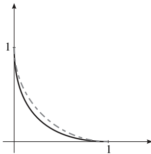
Figure 2. The curve \Gamma (full line) and the arc of circle \mathcal{C} (dashed line)
