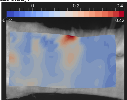
Figure 1: Green Lagrange strain from DIC.
