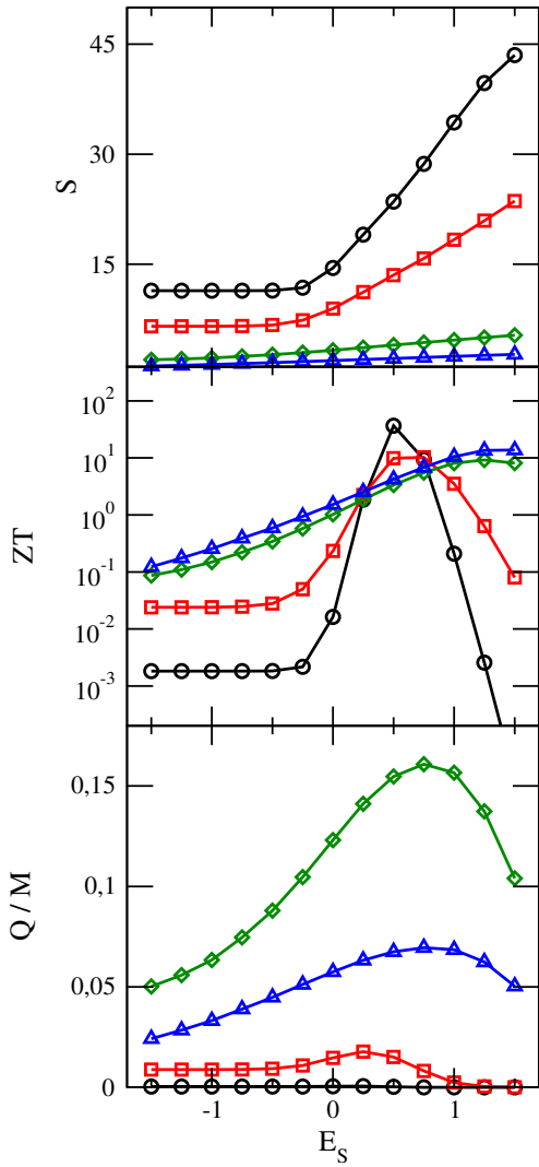
FIG. 5. (Color online) Non local thermopower S (in units of k_B/e ), electronic figure of merit ZT (in units of k_B^2/h ) for various temperatures [ k_B T/\epsilon = 0.05 ( \circ ), 0.1 ( \square ), 0.5 ( \diamond ) and 1 ( \triangle )]. Data are plotted for the hybrid configuration as functions of the (right) barrier height E_s^R \equiv E_s (in units of \epsilon ). Other parameters are E_d = -\epsilon , \Gamma = \epsilon , \gamma_e = \epsilon/\hbar , and \mu = 0 .
