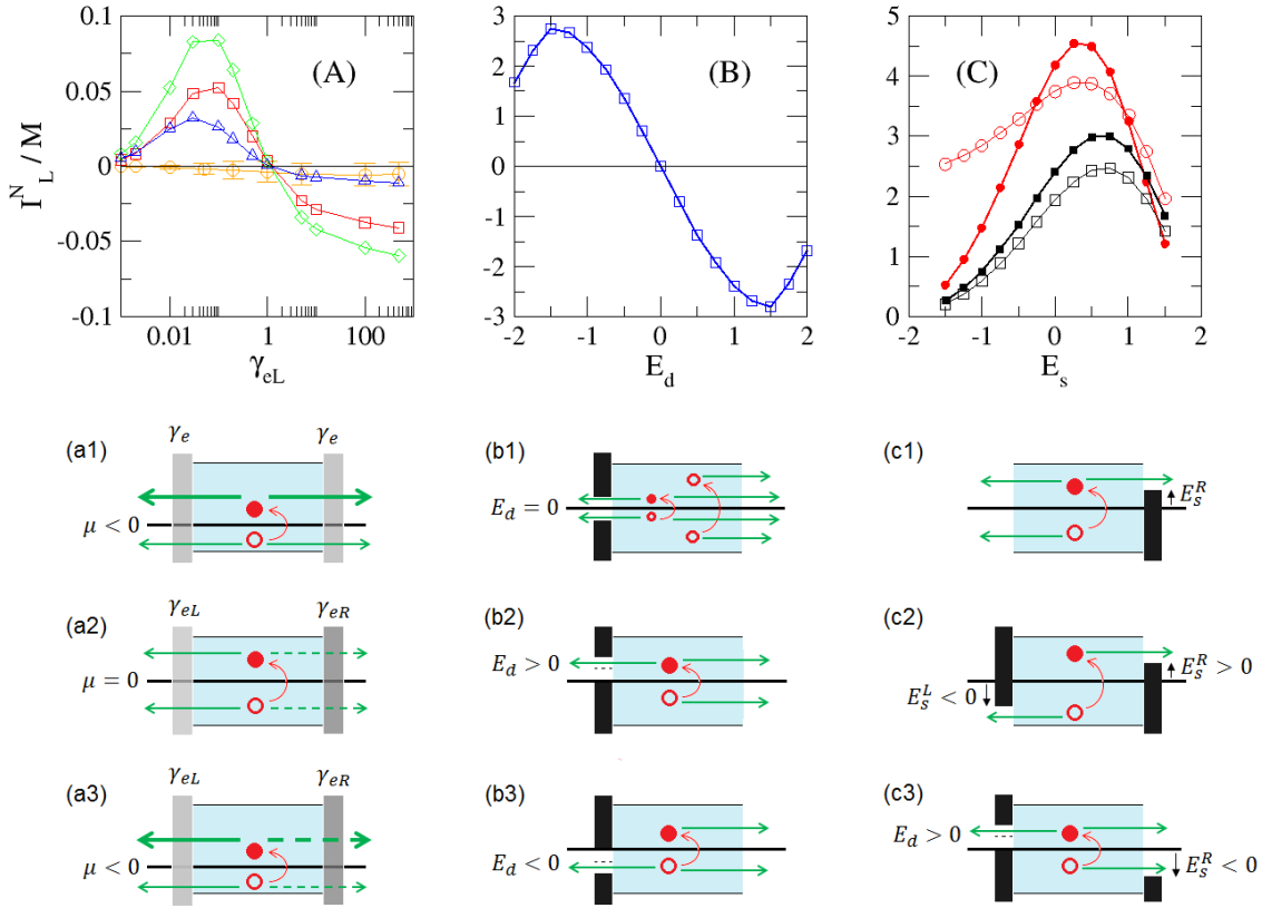
FIG. 2. (Color online) Illustration of the ratchet effect powered by \delta T_P > 0 , for various types of contacts. Particle currents I_L^N (in units of 10^5 \epsilon / \hbar ), obtained with \delta T_P = 10^{-3} \epsilon and \delta \mu = 0 , are plotted in top panels (A-C) for different configurations shown below (a1-c3). (Left) Energy-independent tunnel barriers. If the contacts are symmetric (a1) or if \mu = 0 (a2), I_L^N = 0 on average. If both symmetries are broken (a3) a net current is generated. (A) I_L^N/M as a function of \gamma_{eL} (in units of \epsilon/\hbar ) for fixed \gamma_{eR} = \epsilon/\hbar and various positions of \mu ( \mu/\epsilon = 0 ( \circ ), -0.5 ( \square ), -1 ( \diamond ) and -2.5 ( \triangle )). (Middle) Energy filter. When E_d = 0 electron-hole symmetry makes the total current vanish (b1), whereas E_d > 0 (b2) and E_d < 0 (b3) correspond to negative and positive current, respectively. (B) I_L^N/M at \mu = 0 , for \gamma_{eR} = \epsilon/\hbar on the right and an energy filter on the left with \gamma_e = \epsilon/\hbar , opening \Gamma = \epsilon , and tunable E_d (in units of \epsilon ). (Right) (c1) Single barrier configuration. The Schottky barrier prevents hole-like excitations with energy below E_s^R to escape to the right contact. (c2) Double barrier configuration. A low energy filter is added at the left contact, forbidding electron-like excitations with energy above E_s^L to tunnel leftward. (c3) Hybrid configuration. A Schottky barrier on the right is combined with an energy filter on the left. (C) I_L^N/M at \mu = 0 , as a function of the barrier height E_s (in units of \epsilon ), with \gamma_e = \epsilon/\hbar , for the single barrier ( \blacksquare , E_s \equiv E_s^R ), double barrier ( \bullet , E_s \equiv E_s^R = -E_s^L ), and hybrid cases ( E_s \equiv E_s^R ) with E_d = 0 ( \square ) and E_d = -\epsilon ( \circ ).
