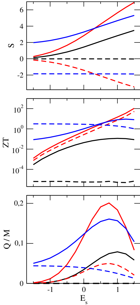
FIG. 6. (Color online) Non local (full lines) versus local (dashed lines) transport coefficients, shown for the single barrier (black), double barrier (red) and hybrid (blue) configurations. Data are plotted as functions of the (right) barrier height E_s^R \equiv E_s (in units of \epsilon ). For the double barrier case, E_s^R = -E_s^L . For the hybrid one, E_d = -\epsilon and \Gamma = \epsilon . The thermopowers and power factors are given in units of k_B/e and k_B^2/\hbar respectively. In all panels, \gamma_e = \epsilon/\hbar and \mu = 0 .
