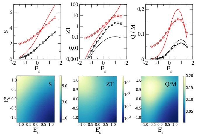
FIG. 3. (Color online) (Top) Non local thermopower S (in units of k_B/e ), electronic figure of merit ZT , and power factor Q (in units of k_B^2/\hbar in the single barrier (black line), double barrier (red line) and hybrid (with E_d = 0 ( \circ ) and E_d = -\epsilon ( \square )) configurations. Data are plotted as functions of the (right) barrier height E_s^R \equiv E_s (in units of \epsilon ). For the double barrier case, E_s^R = -E_s^L . For the hybrid one, \Gamma = \epsilon . (Bottom) S , ZT , and Q/M in the double barrier configuration as functions of the left and right barrier heights E_s^L and E_s^R (in units of \epsilon ). In all panels, \gamma_e = \epsilon/\hbar and \mu = 0 .
