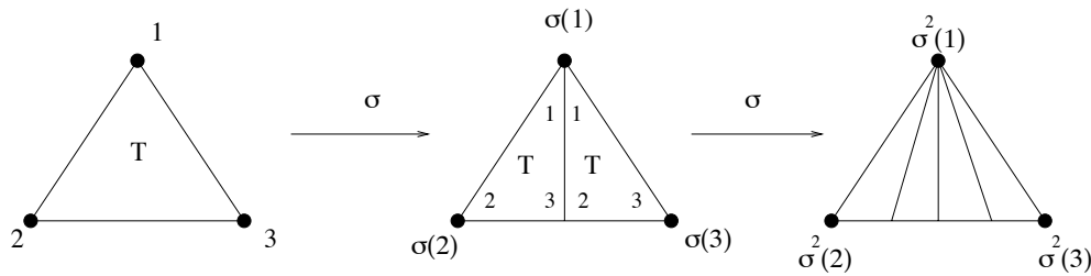
Figure 8: The vertex 1 of the tile T of the above substitution is a divided vertex. The valence of \sigma^k(1) in \sigma^k(T) is 2^k + 1
