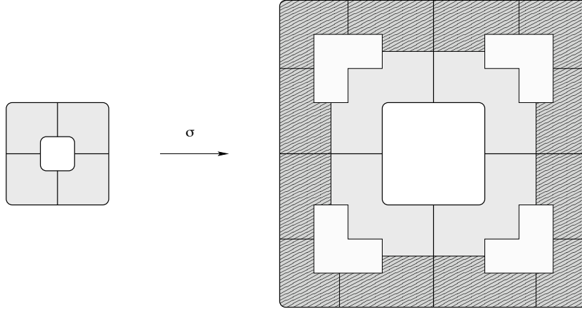
Figure 7: The thick boundary of \sigma^k(T) (hatched on the picture) is contained in the union of the thick boundaries of the images of the tiles in the thick boundary of \sigma^{k-1}(T) (in grey on the picture).
