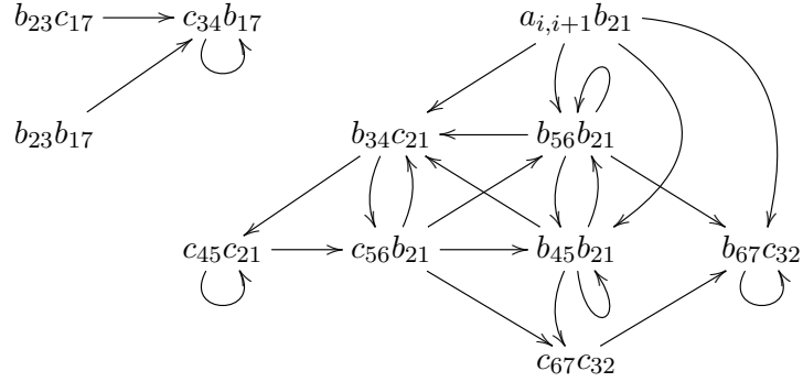
Figure 14: \mathcal{E}(\beta) for the heptagonal substitution
