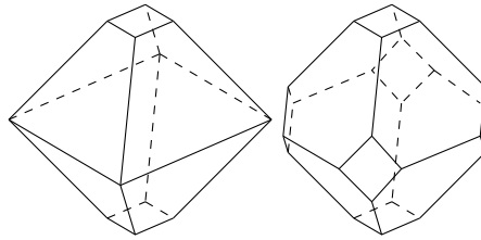
Figure 3: Polytopes Q_n
