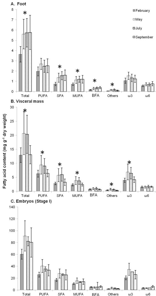
Figure 3. Seasonal variations of fatty acid content of females and embryos (stage I). Seasonal variations of fatty acid content (Total FA, PUFA, SFA, MUFA, BFA, Others, ω3 and ω6) at four periods of the reproductive season of Crepidula formicata (February, May, July and September). A: foot; B: visceral mass; C: embryos (stage I). Histograms represent means and error bars correspond to standard deviations. Black stars represent significant differences between periods (Kruskal-Wallis test, p < 0.05 ).
