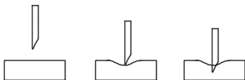
Figure 2: the three stages of needle-soft tissue interaction model
