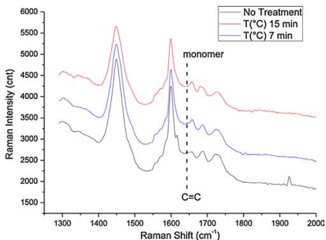
Fig. 2. Raman spectra of a 10 \mu\text{m} encapsulated droplets obtained with Inj-1 system after a thermal (115 °C) post-treatment.
