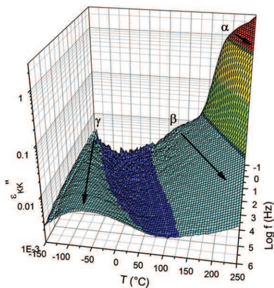
Fig. 6. \epsilon''_{KK} deduced from \epsilon'_{T(\omega)} by analytical Kramer–Kronig transform.
