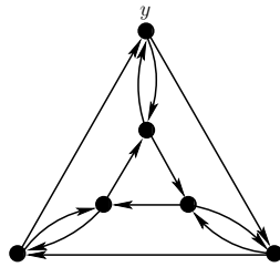
Fig. 1: The smallest planar hypohamiltonian digraph
