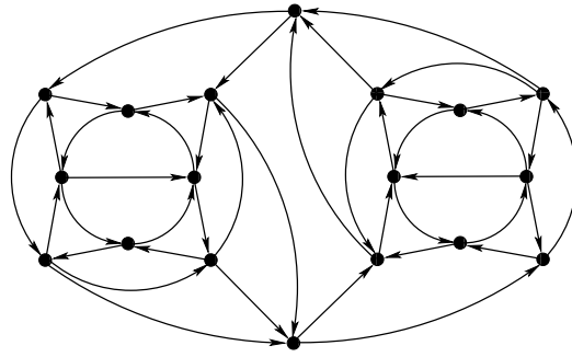
Fig. 8: A strong planar hypotractable oriented graph of order 18
