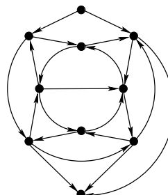
Fig. 4: A planar hypotraceable oriented graph of order 10
