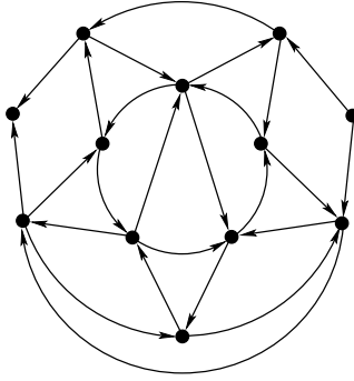
Fig. 7: A planar hypotraceable oriented graph of order 12
