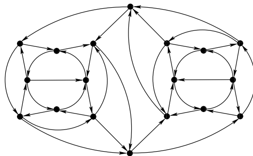
Fig. 8: A strong planar hypotraceable oriented graph of order 18
