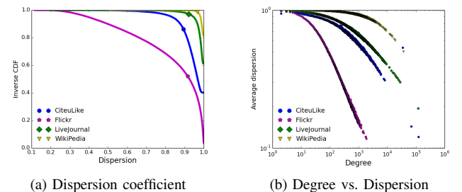
Fig. 8. Inverse cumulative distribution of the dispersion coefficient and correlation between degree and dispersion for random networks with the same \top and \perp degree distributions.
