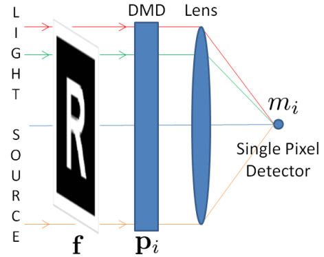
Fig. 1. Optical setup composed of a DMD and a single pixel detector. The measure at the detector corresponds to the projection of the image on a certain pattern.
