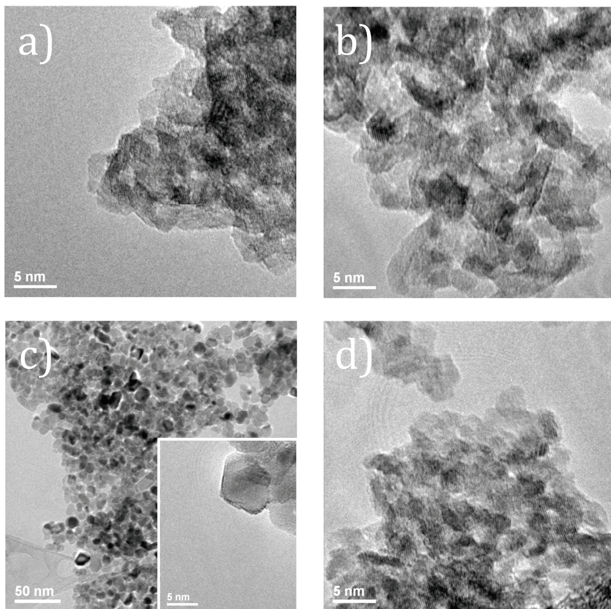
Fig 3. TEM images of a) \text{Ni}_3\text{O}_2(\text{OH})_4 ; b) \text{NiO-250} ; c) \text{NiO-500} ; d) \text{NiO-N-250} samples.
