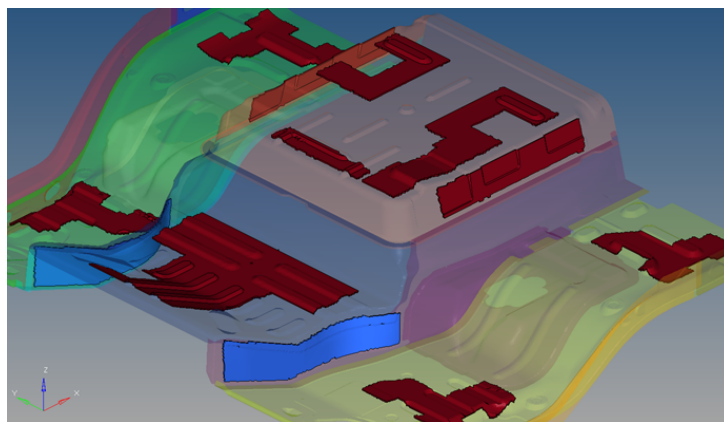
Figure 3: FEM floor model with viscoelastic patches.
