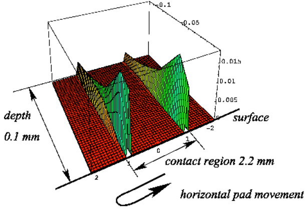
Fig. 5 Typical spatial distribution of the equivalent plastic strain (vertical axis) in the refined part of the mesh after the 40th loading cycles (combined hardening, P = 7.5 kN, \delta = 12.0 \mu m and \mu = 0.3 ).
