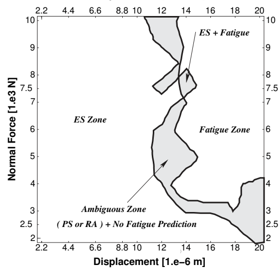
Fig. 19 Theoretical domain of applicability of the Dang Van criterion (ES, i.e. elastic shakedown domain) versus predicted fatigue domains for Titanium: isotropic hardening (top), kinematic hardening (middle), combined hardening (bottom).
