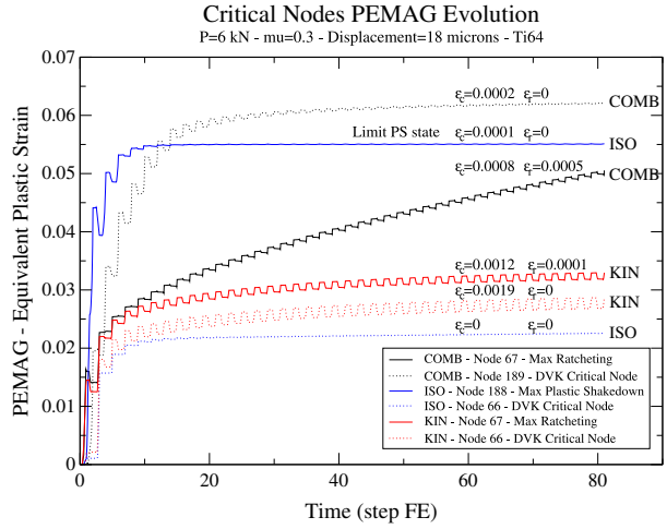
Fig. 10 Evolution of plastic strain in a ratcheting case for the different constitutive models (kinematic, KIN; isotropic, ISO; and combined, COMB) of Ti64.
