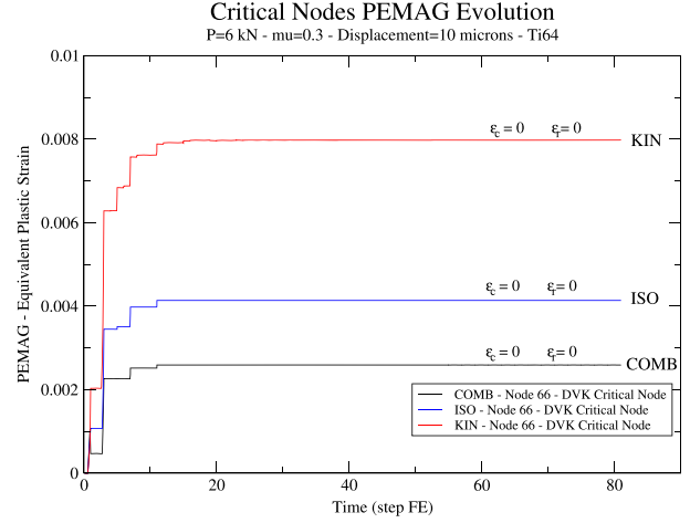
Fig. 8 Evolution of plastic strain in a case of elastic shakedown, for the three different constitutive models (kinematic, KIN; isotropic, ISO; and combined, COMB).
