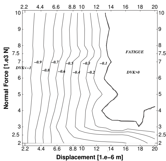
Fig. 18 Contours plots of the Dang Van criticality for \mu = 0.3 and for the three different constitutive models of Titanium: isotropic hardening (top), kinematic hardening (middle) and combined hardening (bottom).
