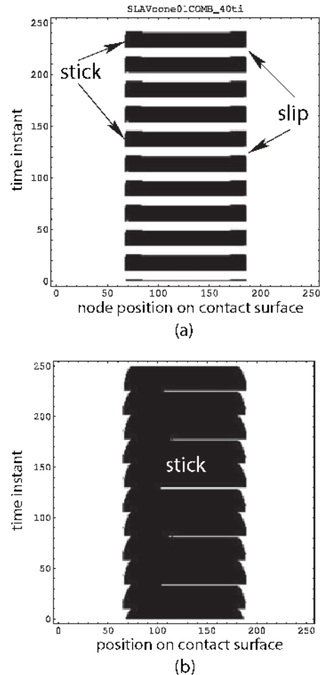
Fig. 13 Stick-slip Plot for Ti64-combined hardening: (a) P=2.5 kN, \mu=0.1 and \delta=11 \mu\text{m} and (b) P=2.5 kN, \mu=0.3 and \delta=6.6 \mu\text{m} (1 cycle = 6 time instants).
