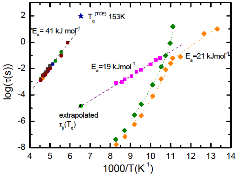
FIG. 9: Relaxation times as a function of temperature. TCE: \beta phase (filled circles), glass phase (■). Dielectric relaxation data for Freon 112 of Pardo et al. (Ref. 17) are also shown: (◆) \alpha -relaxation, (◇) \beta -relaxation.
