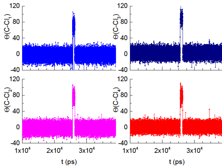
FIG. 8: Reorientation angle of C- Cl (i) bond (i=1- 4).
