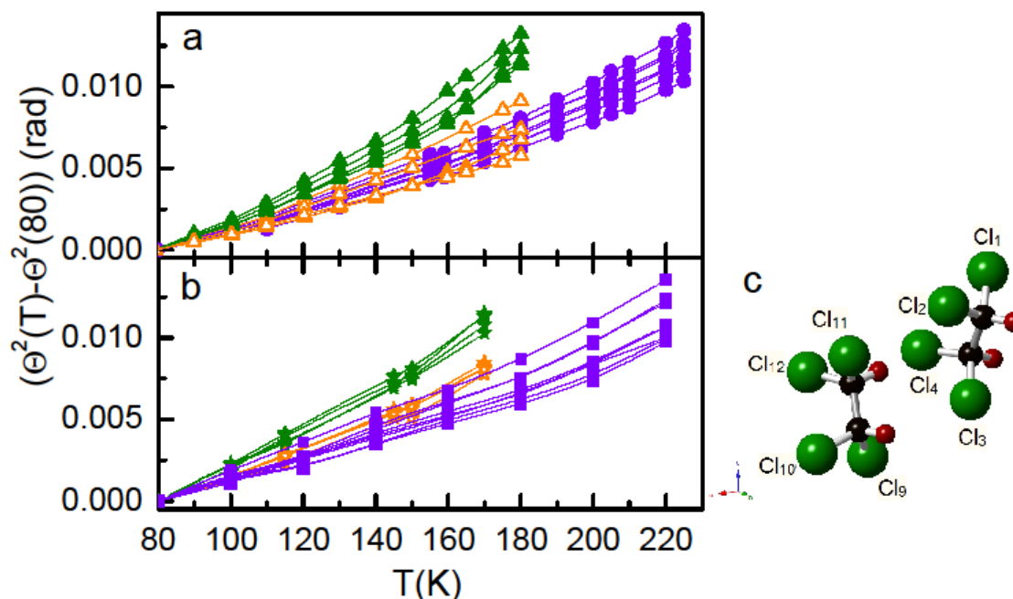
FIG. 5: a) experimental values of \Delta\theta^2 : \beta phase ( \bullet ) and \gamma phase ( \blacktriangle, \triangle ). b) MDS values of \Delta\theta^2 : \beta phase ( \blacksquare ) and \gamma phase ( \star, \star ). ( \star ) correspond to Cl 1 , Cl 3 and Cl 9 , Cl 11 , ( \star ) correspond to Cl 2 , Cl 4 and Cl 10 , Cl 12 as shown in c). Atomic labels according to Ref. 5.
