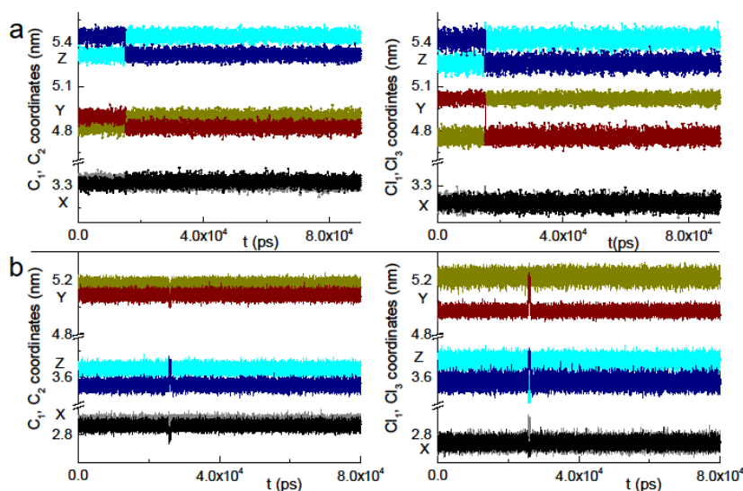
FIG. 7: Carbon and Chlorine coordinates of two different molecules at 230 K, after 300ns of NVT MDS. a) 180^\circ reorientations around the molecular symmetry axis, b) reorientations between non-equivalent positions.
