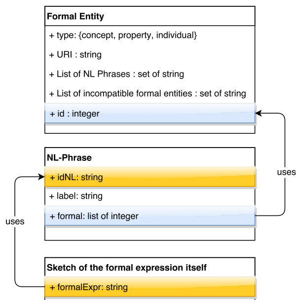
Figure 1: A schematic view of the specifications of BEUFORD.
