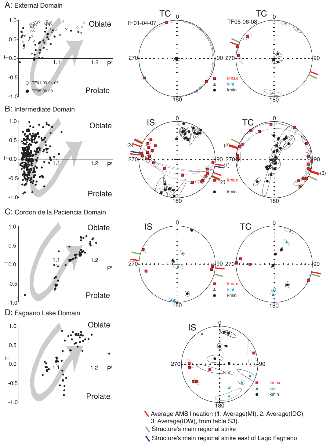
Figure 11. T-P' diagram and equal area stereonets of AMS ellipsoids for several localities in Tierra del Fuego. (a) External domain, (b) intermediate domain, (c) Cordon de la Paciencia, and (d) Lago Fagnano domain. Same legend as in Figure 9 for the AMS plots. The grey-shaded path with arrow illustrates the changes in the parameter T and degree of anisotropy for increasing deformation (from Robion et al. [2007], modified from Borradaile and Henry [1997]). Data supporting Figure 11 is available in the supporting information Table S3.
