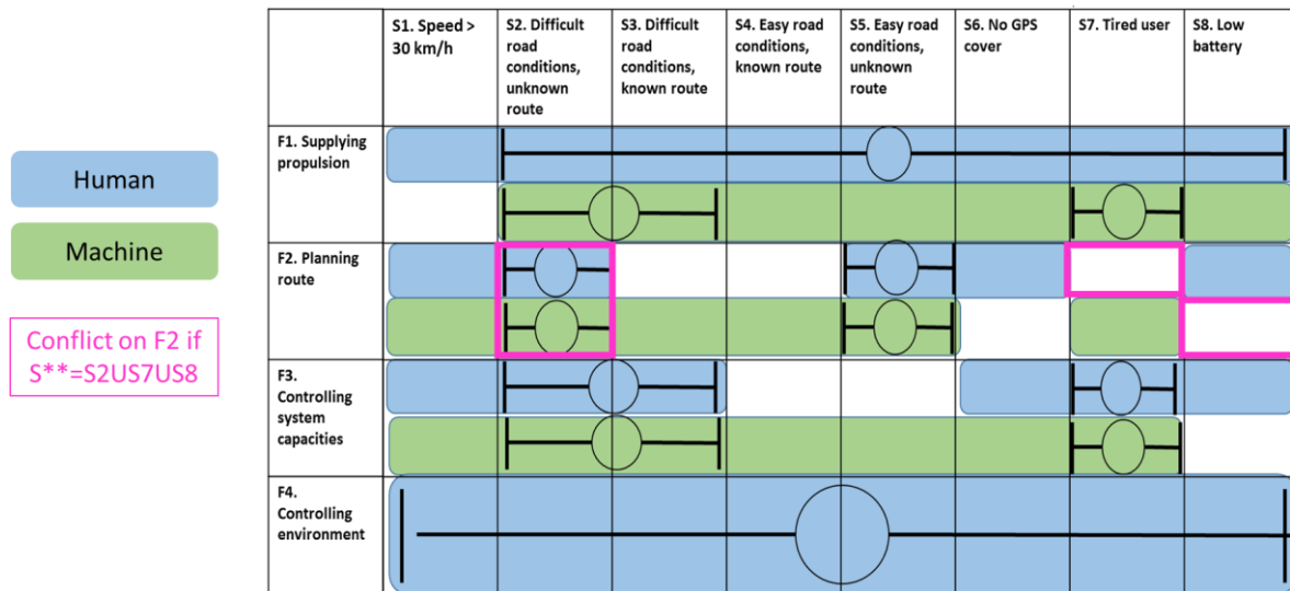
Figure 4: Contextual Activity Template and SOCA-CAT
