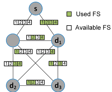
Fig. 2. Spectrum resources on links in an EON.
