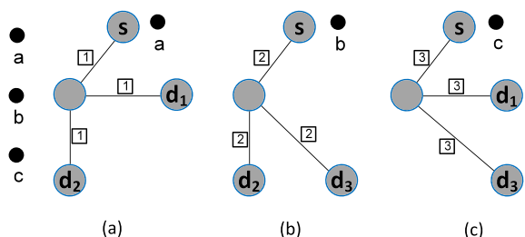
Fig. 4. Example on multicast using light-forest with R-NC.
