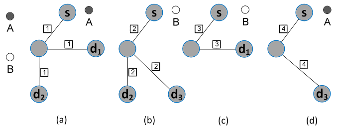
Fig. 3. Example on multicast using light-forest without R-NC.
