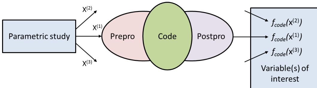
Figure 1: Illustration of the code manager. In a parametric study, all the code simulations are characterized by a finite-dimensional vector \boldsymbol{x} of scalar parameters. The code manager first consists in a preprocessor, which generates code inputs from these parameters. After the simulation, the code manager incorporates a postprocessor, which checks the occurrence of computational failure and then condense the code output in some variables of interest.
