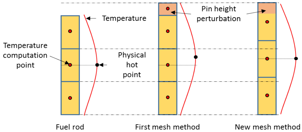
Figure 7: Simplified illustration of the impact of a perturbation of the pin height input on the mesh generation for a Germinal computation. In the original Germinal computations, mild changes of the pin height can cause significant modifications of the mesh, themselves causing the code instabilities of Figure 6. We consequently updated the preprocessor to solve this issue.
