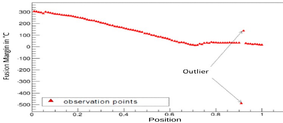
Figure 8: Same settings as in Figure 6, but for the updated Germinal computations. The code instabilities have been corrected.
