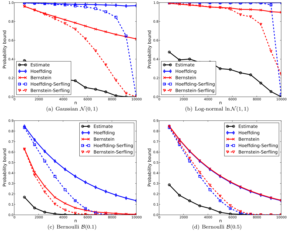
FIG 1. Comparing known bounds on p = \mathbb{P}(n^{-1} \sum_{i=1}^n X_i - \mu \geq 0.01) with our Hoeffding-Serfling and Bernstein-Serfling bounds. \mathcal{X} is here a sample of size N = 10^4 from each of the four distributions written below each plot. An estimate (black plain line) of p is obtained by averaging over 1000 repeated subsamples of size n , taken from \mathcal{X} uniformly without replacement.
