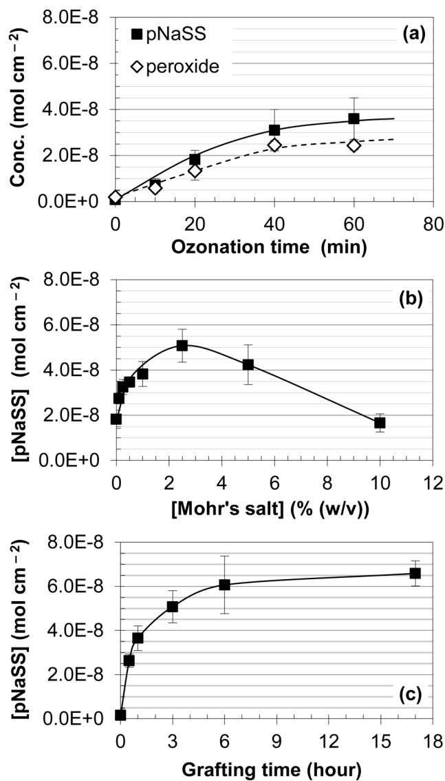
Fig. 1. Concentration of peroxide (◇) or grafted pNaSS (■) on PCL films as a function of various parameters: (a) effect of the ozonation time (grafting time = 3 h, [Mohr's salt] = 0 % (w/v)); (b) effect of the Mohr's salt concentration in the grafting solution (process parameters: ozonation time = 20 min, grafting time = 3 h); (c) effect of the grafting time (process parameters: ozonation time = 20 min, [Mohr's salt] = 2.5 % (w/v))
