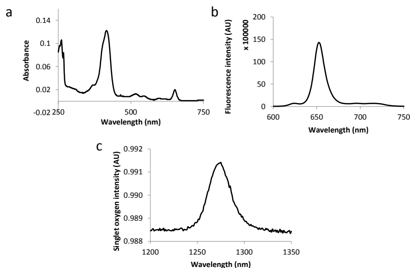
Figure 4. Absorption spectra (a), fluorescence emission (b) and singlet oxygen emission spectra (c) for TPC-PEG9-TKPRR in ethanol.
