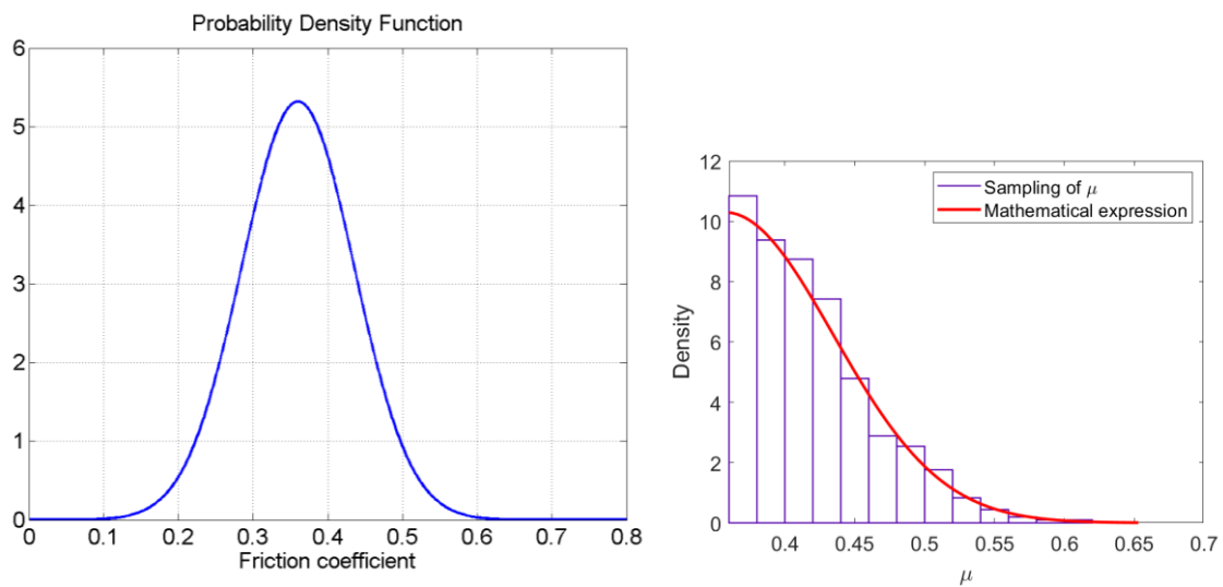
Fig. 4: Statistical distribution of friction coefficient between wheel and rail (right figure added in 2024: should have been used instead of left figure!)
