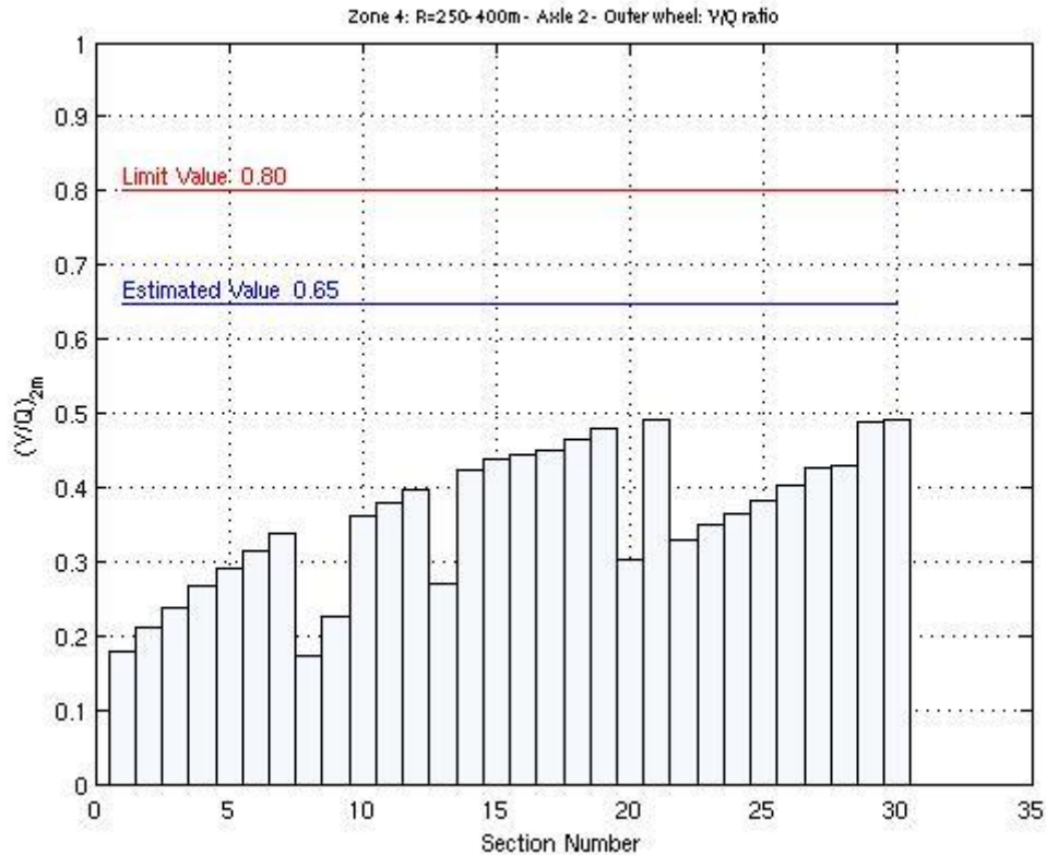
Fig. 2: Percentiles on each section of Y/Q ratio; estimated value based on 30 sections and limit value
