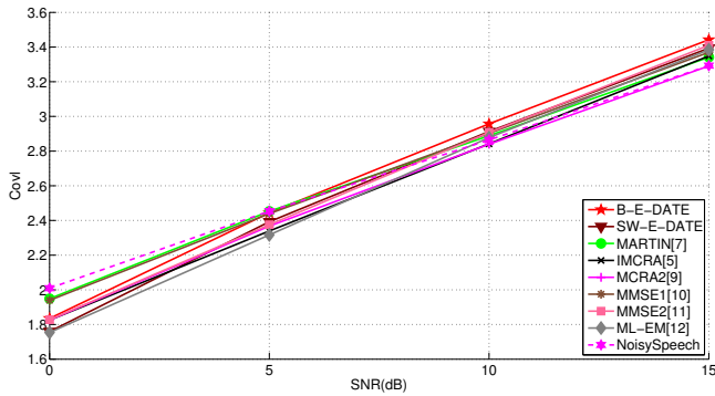
(g) babble noise
