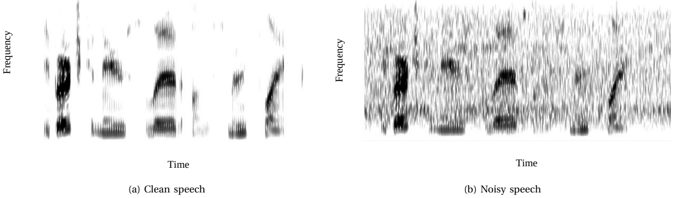
Fig. 1: Spectrograms of clean and noisy speech signals from the NOIZEUS database. The noise source is car noise. No weighting function was used to calculate the STFT.
