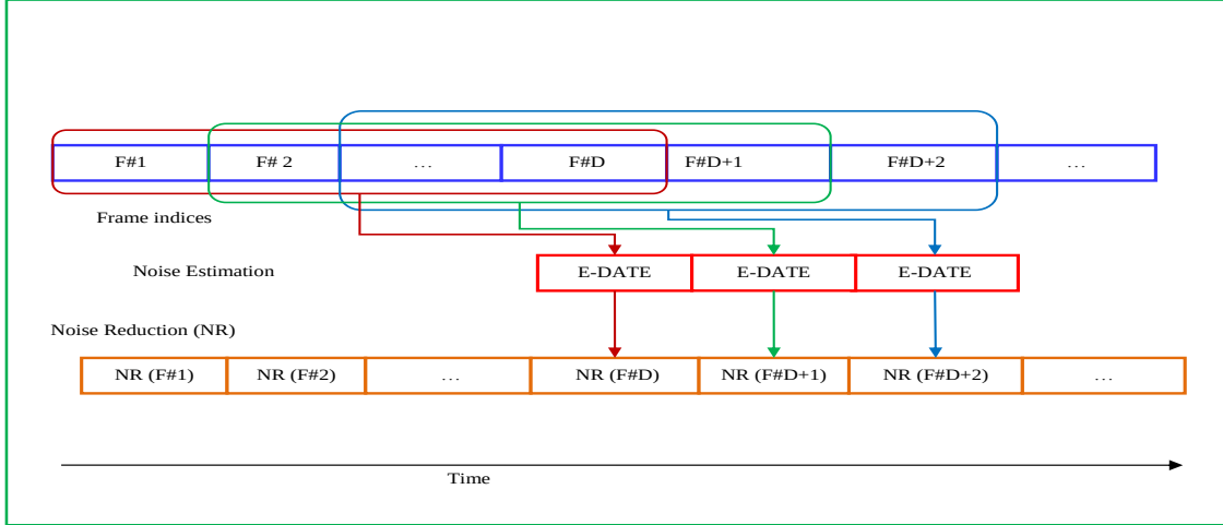
Fig. 4: Sliding-Window E-DATE (SW-E-DATE) combined with noise reduction. For the first D - 1 frames, a surrogate method for noise power spectrum estimation is used in combination with noise reduction. Once D frames are available and upon reception of frame D + \ell , \ell \geq 0 , the SW-E-DATE algorithm provides the NR system with a new estimate of the noise power spectrum computed using the last D frames F_{\ell+1}, \dots, F_{\ell+D} for denoising of the current frame.
