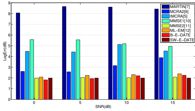
(c) car noise
