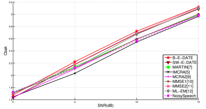
(b) airport noise
