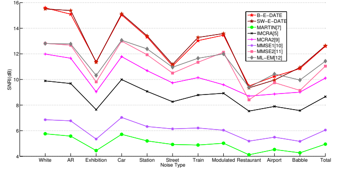
Fig. 6: SNRI with various noise types
