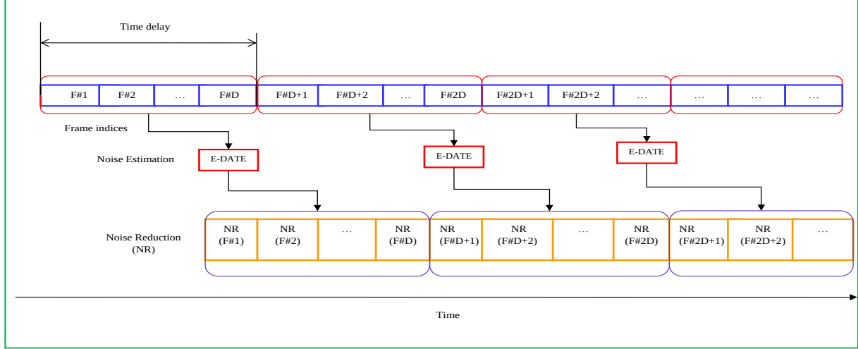
Fig. 3: Block E-DATE (B-E-DATE) combined with noise reduction (NR). A single noise power spectrum estimate is calculated every D non-overlapping frames and used to denoise each of these D frames.
