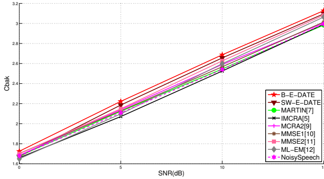
(a) babble noise
