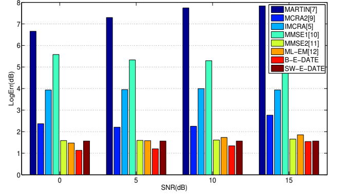
(b) AR noise
