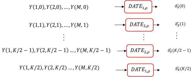
Fig. 2: Principle of noise power spectrum estimation based on the DATE in colored stationary noise
