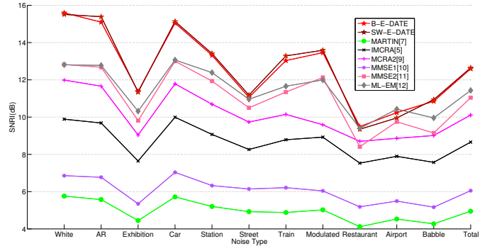
Fig. 6: SNRI with various noise types
