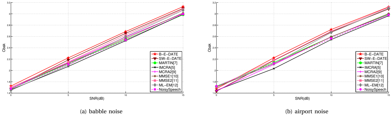
Fig. 8: Speech quality evaluation after speech denoising ( C_{bak} composite criterion).
