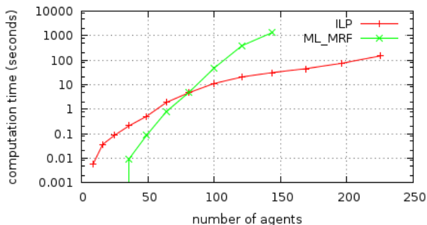
Figure 2: Computation average times for the PNE problem in square grids made of 2 actions agents.
