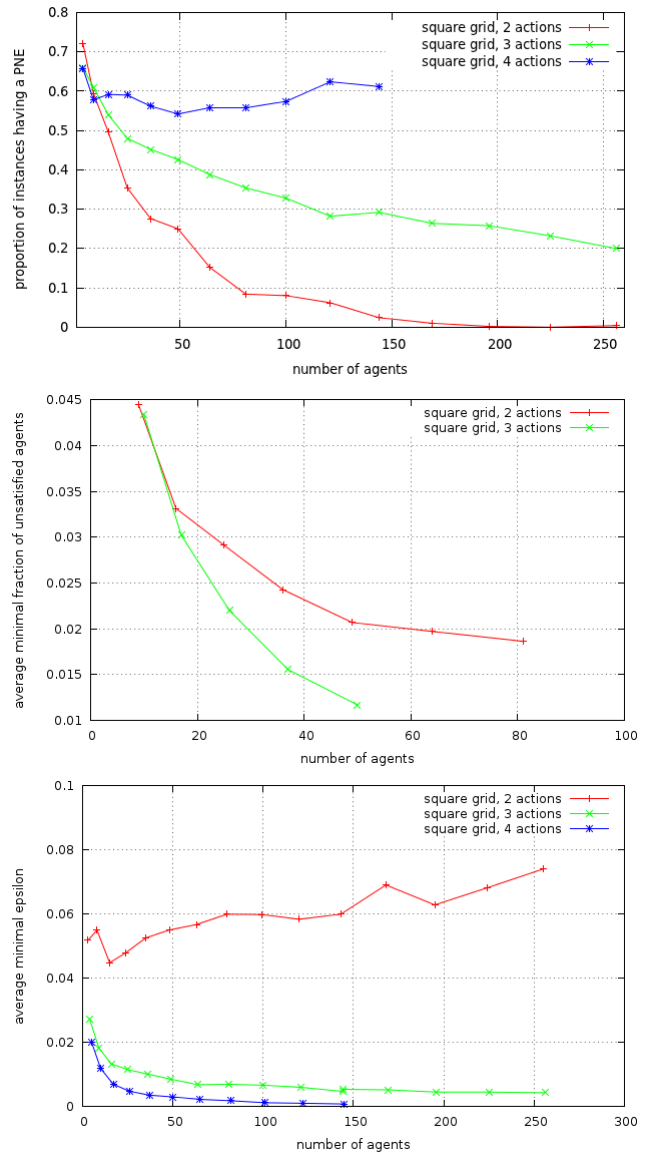
Figure 4: Indicators of PNE proximity in random-payoff GG : square grid graph
