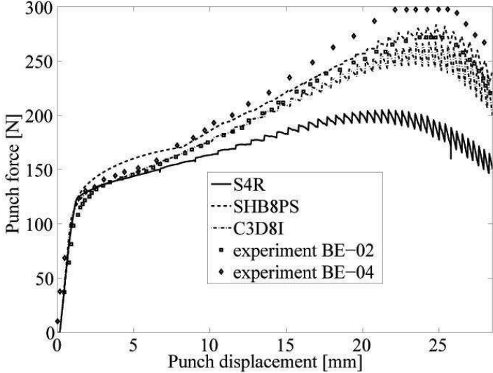
Figure 6: Punch force vs. punch displacement curves for High Strength Steel
