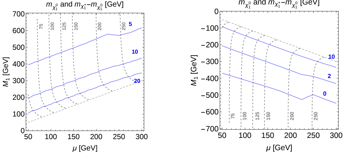
Figure 2. Mass splitting between \tilde{\chi}_1^\pm and \tilde{\chi}_1^0 (blue solid line) and mass of \tilde{\chi}_1^0 (gray dashed line) in the \mu - M_1 plane.
