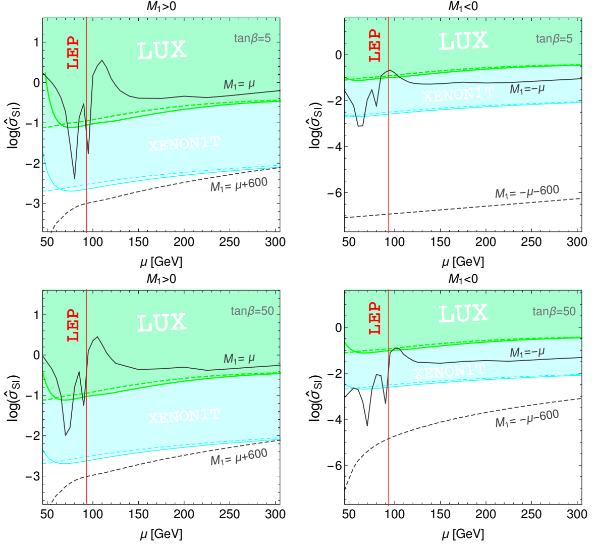
Figure 4. The logarithm of the predicted value of the spin-independent annihilation cross section for DD \hat{\sigma}_{\text{SI}} = R_{\Omega} \sigma_{\text{SI}} / (10^{-8} \text{ pb}) , rescaled by R_{\Omega} / (10^{-8} \text{ pb}) where R_{\Omega} = \Omega_{\text{DM}} / \Omega_{\text{DM}}^{\text{Planck}} , is shown as a function of \mu for \tan\beta = 5, 50 and positive (left) or negative (right) values of M_1 as indicated. The excluded limit from LUX (green), as well as the projected exclusion from XENON1T (cyan) are also shown for comparison, where the solid and dashed lines represent the exclusions for |M_1| = \mu and |M_1| = \mu + 600 GeV respectively.
