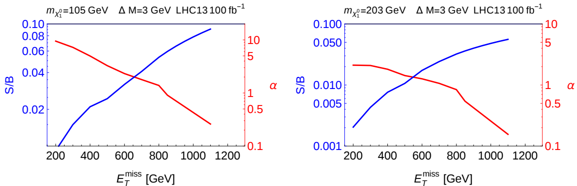
Figure 10. S/B and \alpha as a function on the final selection cut on the E_T^{\text{miss}} for \tilde{\chi}_1^0 \sim 100 GeV (left panel) and \sim 200 GeV (right panel).
