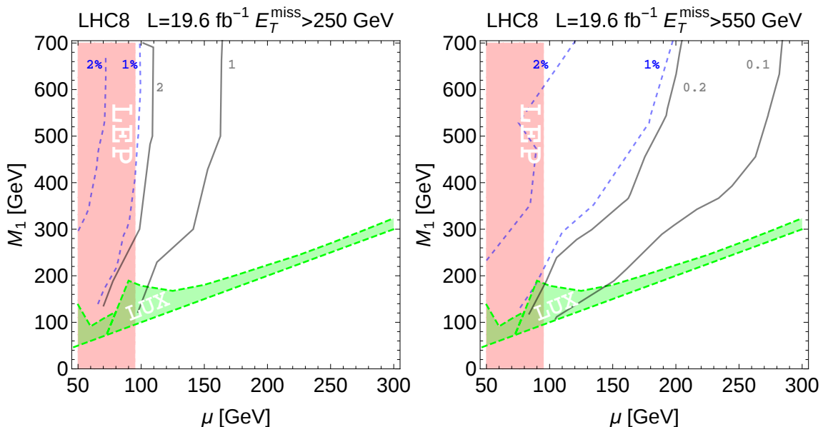
Figure 8. Contours for the 2(\sqrt{S+B} - \sqrt{B}) (gray) and S/B (blue-dashed) in the plane (\mu, M_1) for the signal regions 1 and 7 as defined in [105]. LUX and LEP exclusions are shown in green and red.
