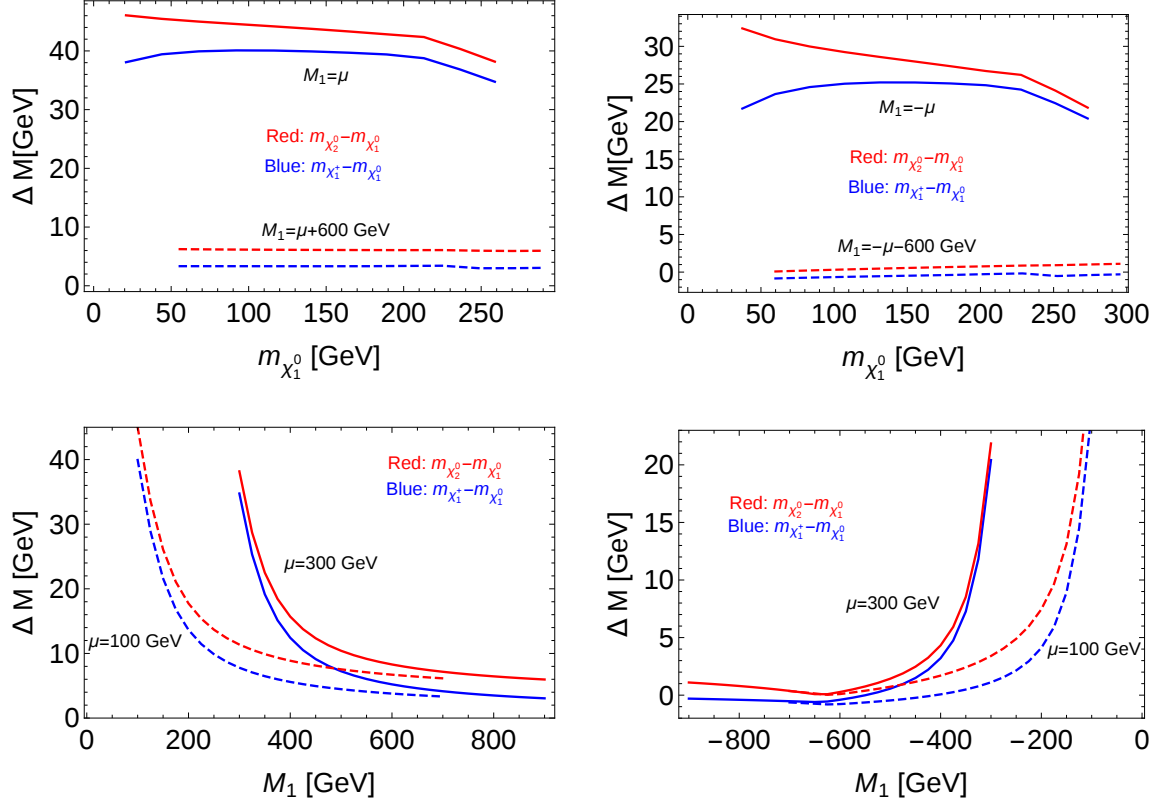
Figure 1. \tilde{\chi}_1^\pm - \tilde{\chi}_1^0 and \tilde{\chi}_2^0 - \tilde{\chi}_1^0 mass splitting values as a function of m_{\chi_1^0} (upper row) and M_1 (lower row) for the case M_1 > 0 (left) and M_1 < 0 (right).
