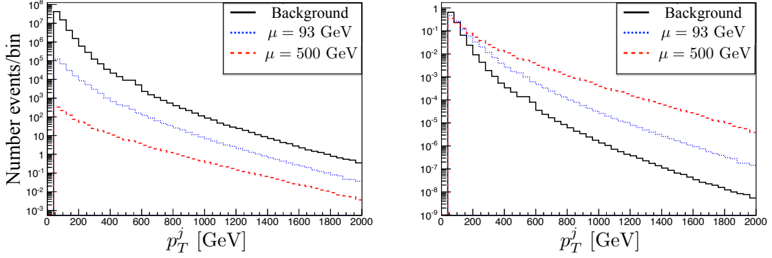
Figure 9. Signal (dotted blue and dashed red) and Zj background (solid black) parton-level p_T^j distributions for the 13 TeV LHC for the NSUSY scenario. Left: p_T^j distributions for 100 \text{ fb}^{-1} integrated luminosity. Right: normalised signal and Zj background distributions.
