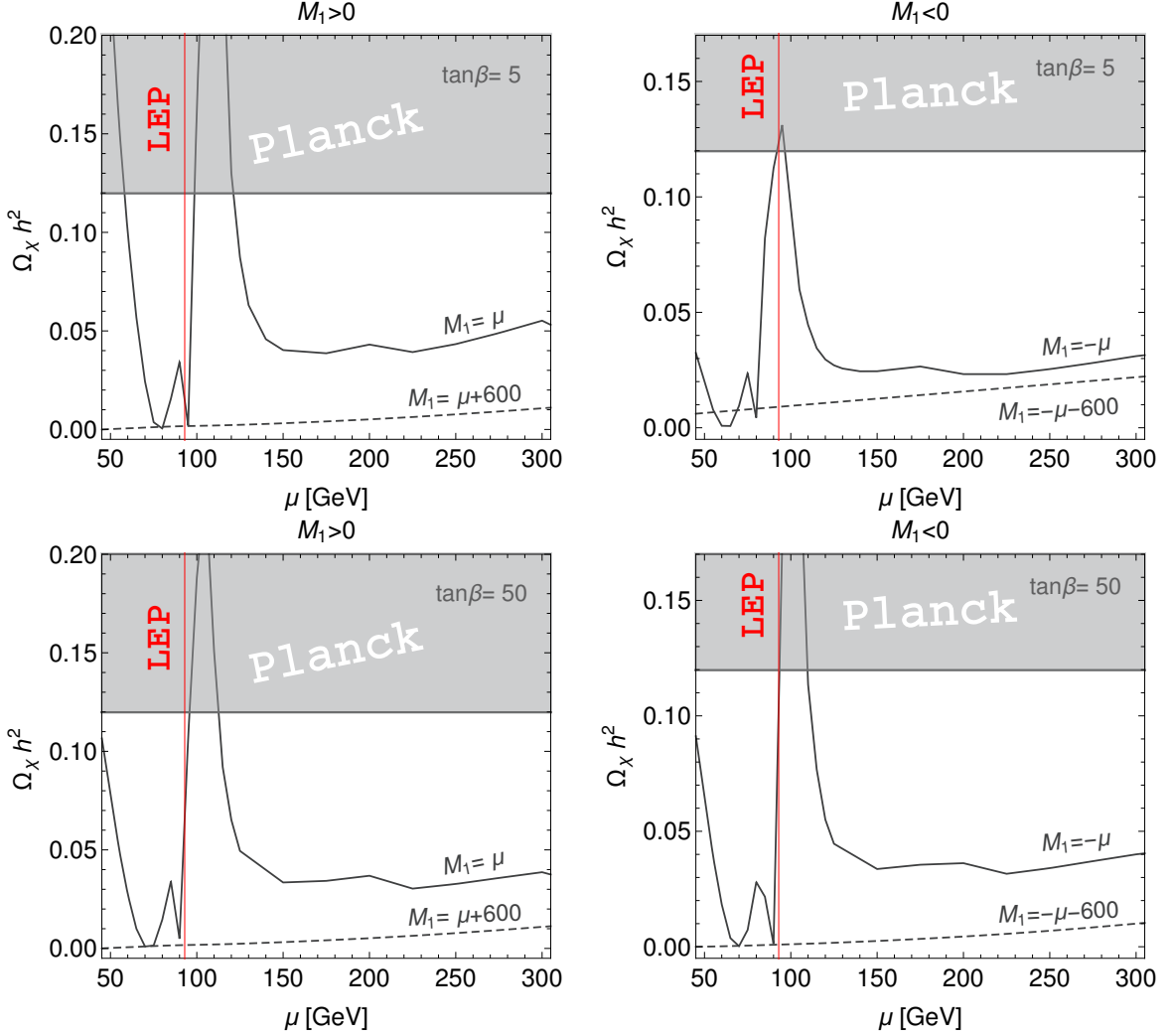
Figure 3. The predicted value of the dark matter relic density \Omega_{\text{DM}} h^2 is shown as a function of \mu for \tan\beta = 5, 50 and positive (left) or negative (right) values of M_1 as indicated. The relic density measured by the Planck satellite, \Omega_{\text{DM}}^{\text{Planck}} h^2 , is also shown for comparison, and the region excluded due to an overabundance of DM is indicated in grey.
